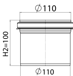
Bunn \varnothing 110
