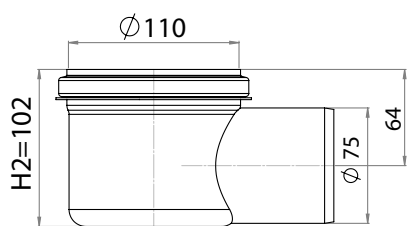
Side \varnothing 75
